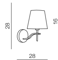
Princessa wall AZ0723 E14 1x 40W metal/chrome/fabric
